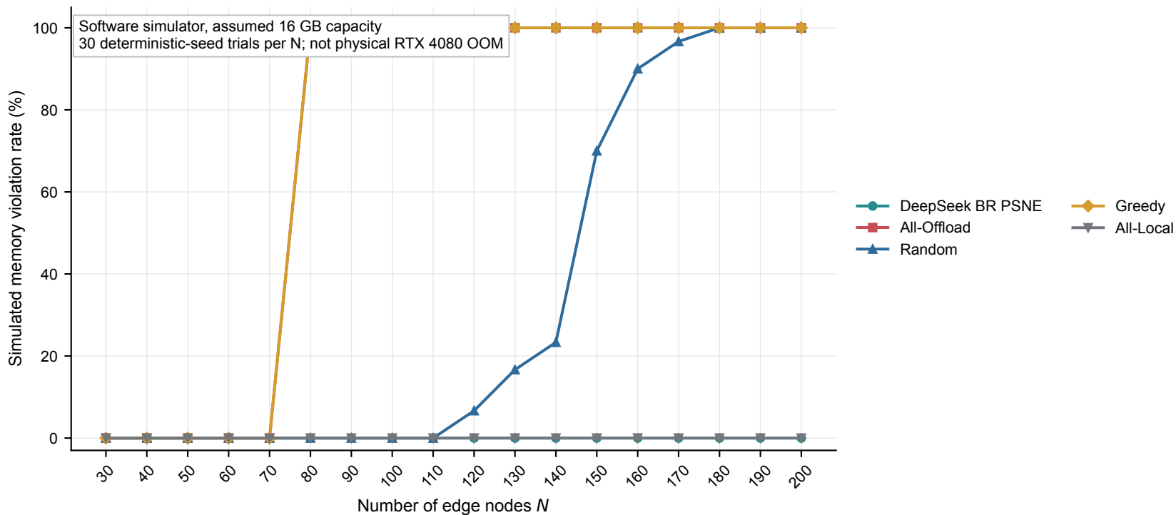
Memory-capacity violations across the PDF-required N = 30 -200 sweep
