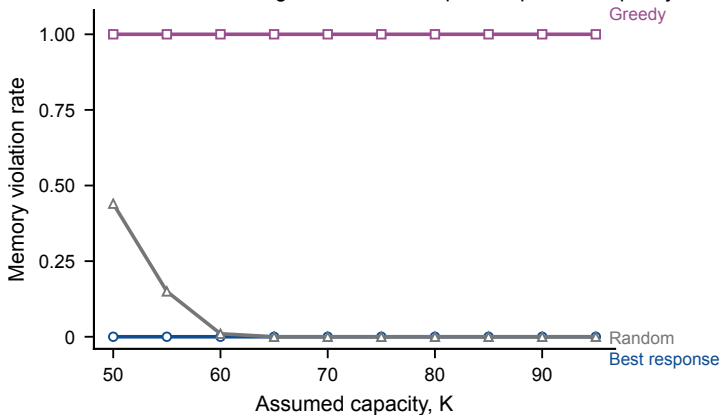
Mark2 Alibaba: congestion-aware responses prevent capacity violations
