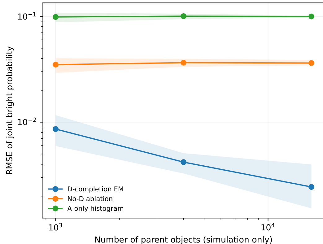
Accuracy of observable bivariate probabilities \rho = 0.55 ; deep; 20 independent parent catalogues
