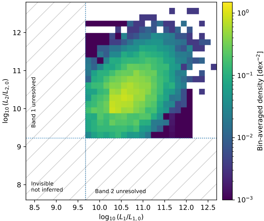
Ablation: no truncation correction \rho = 0.55 ; deep design
