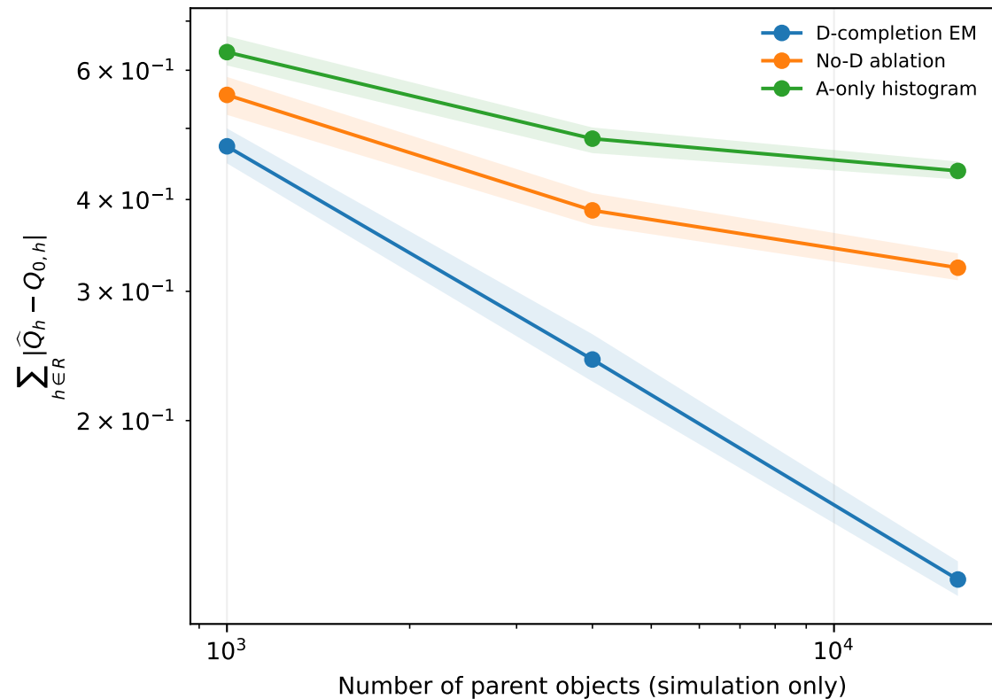
Recovery of resolved luminosity-bin masses \rho = 0.55 ; deep; 20 independent parent catalogues
