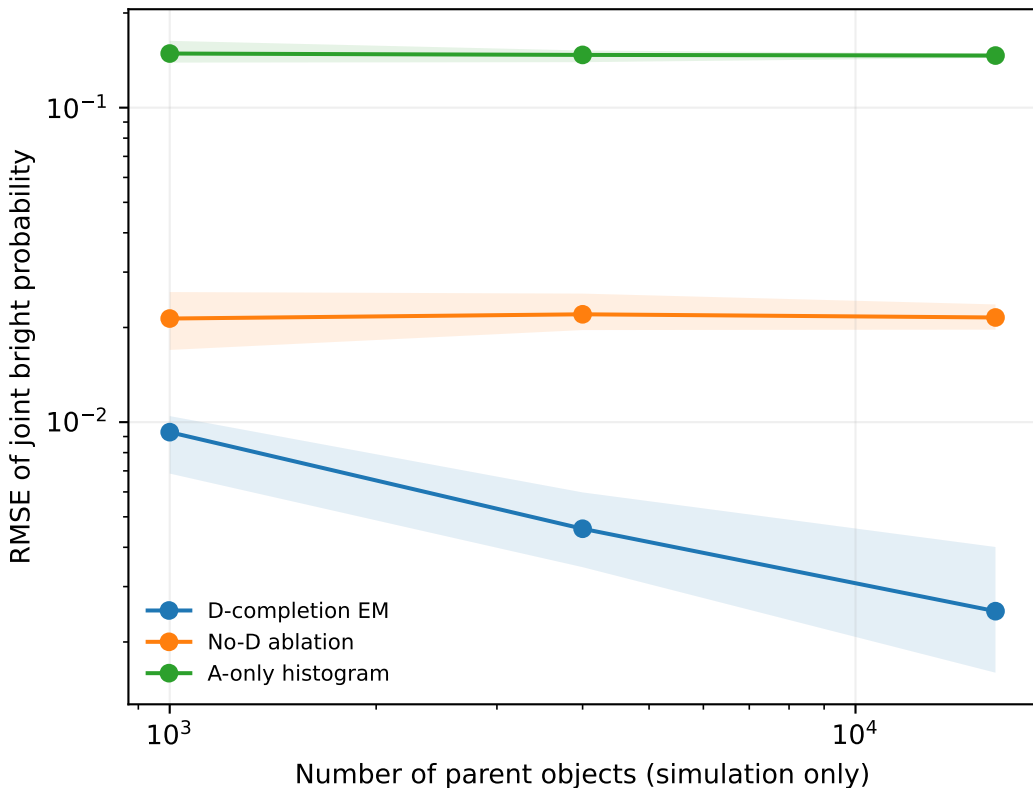
Accuracy of observable bivariate probabilities \rho = 0.55 ; shallow; 20 independent parent catalogues
