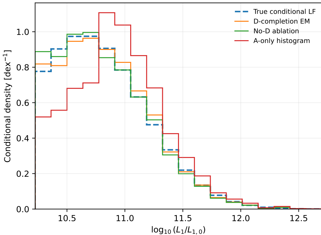
Luminosity marginal in common resolved region \rho = 0.55 ; shallow
