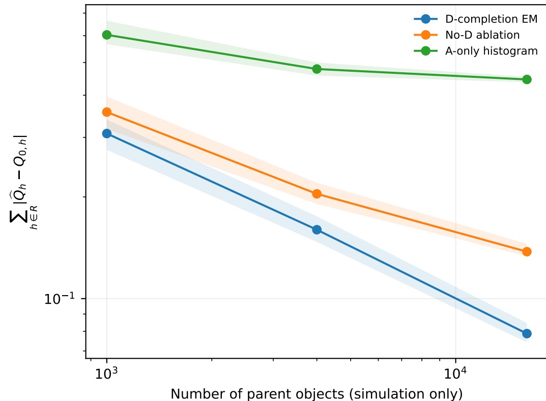
Recovery of resolved luminosity-bin masses \rho = 0.55 ; shallow; 20 independent parent catalogues
