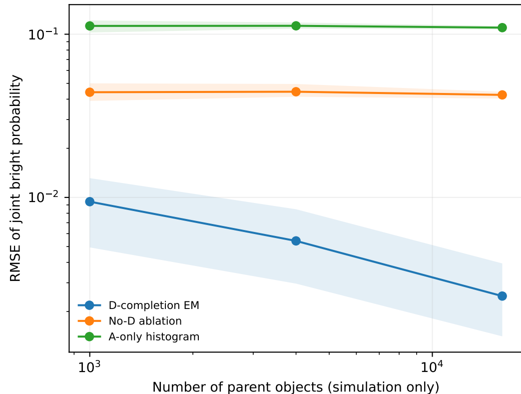
Accuracy of observable bivariate probabilities \rho = 0.90 ; deep; 20 independent parent catalogues
