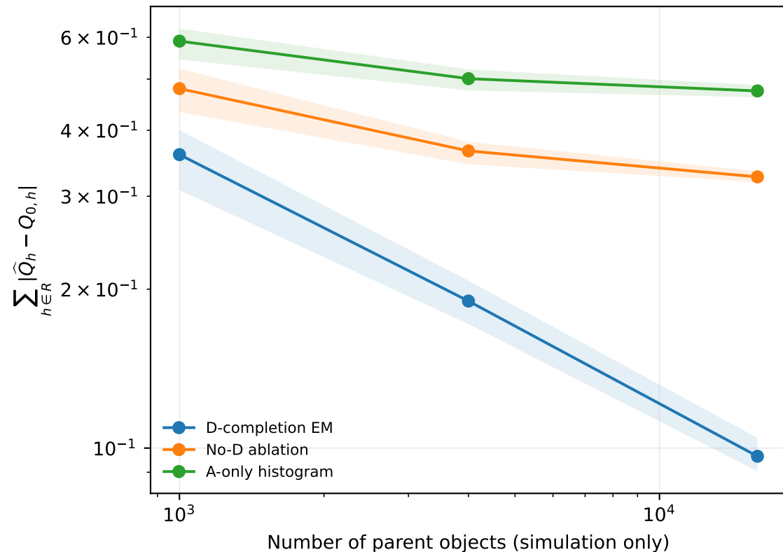
Recovery of resolved luminosity-bin masses \rho = 0.90 ; deep; 20 independent parent catalogues
