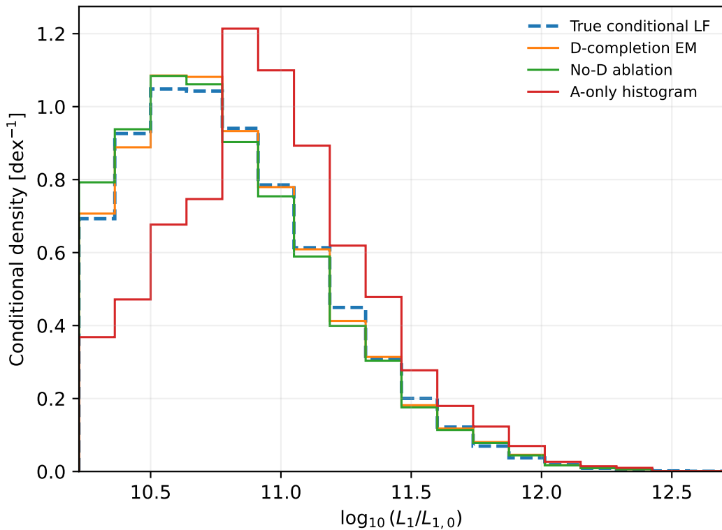
Luminosity marginal in common resolved region \rho = 0.90 ; shallow
