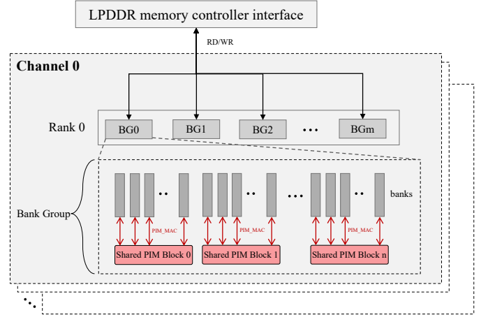
Fig. 1. LPDDR-PIM architecture based on Samsung’s release [?]. A SIMD PIM block sits near the bank I/O and is driven by PIM commands. Samsung specifies two organizations: one PIM block per bank ( b=1 ), or one block shared across a two-bank group ( b=2 ).
