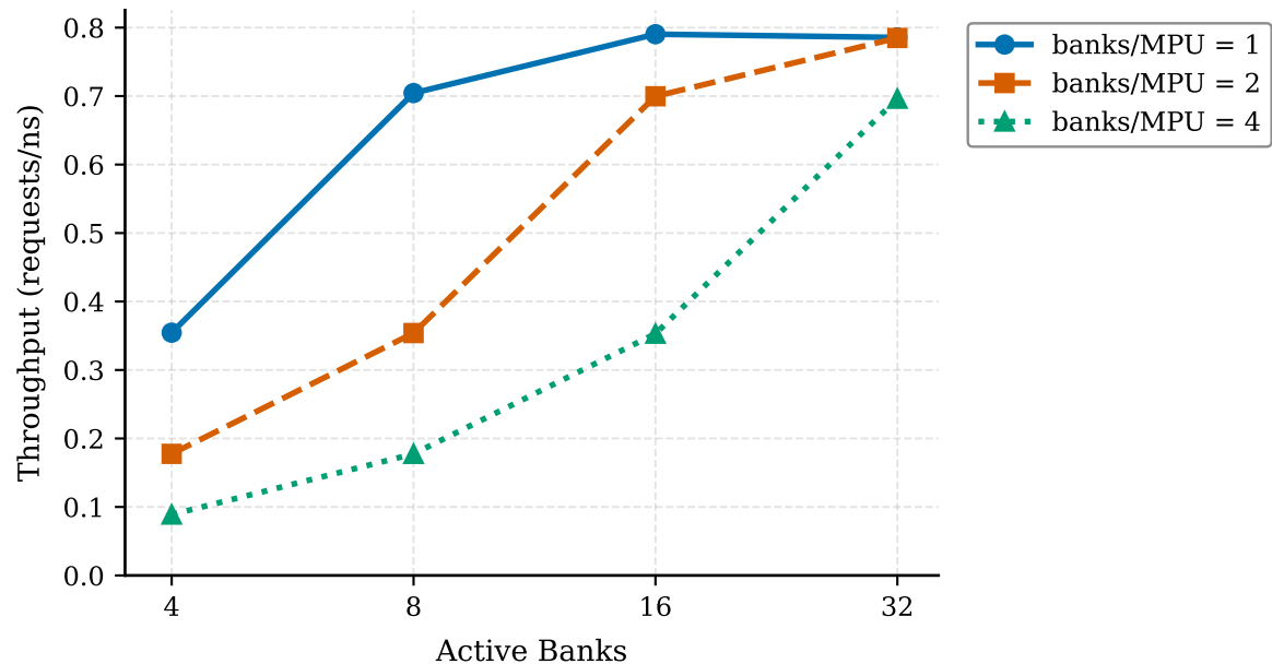
PIM Throughput vs Active Banks (NOP=1)
