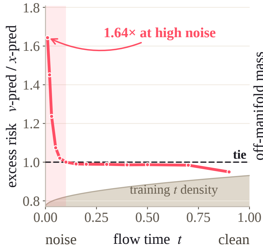
The gain is where sampling starts
