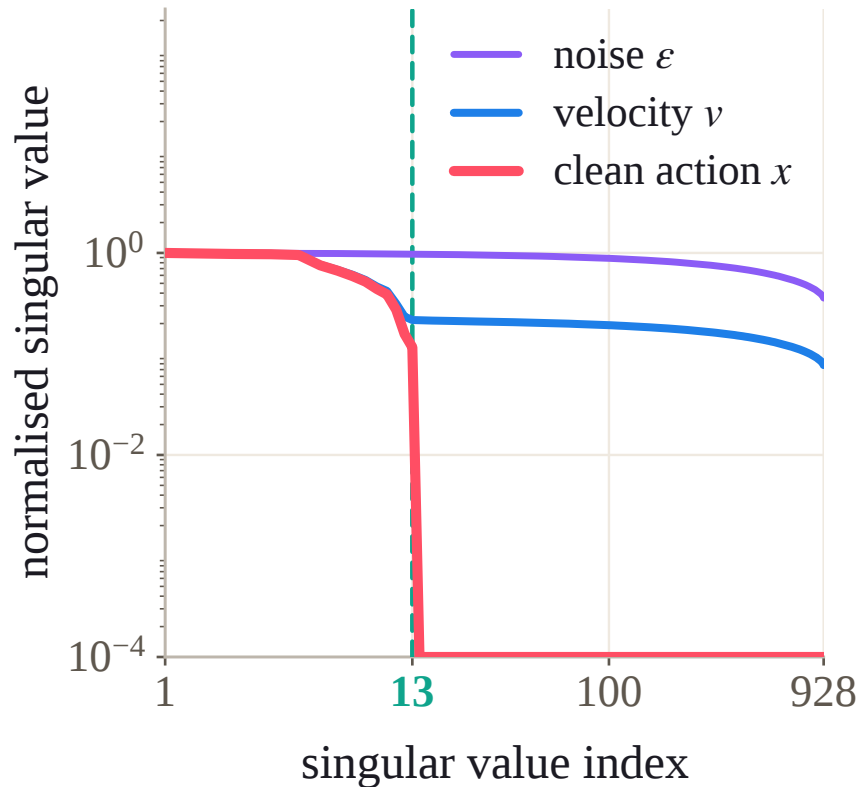
Clean actions are low-dimensional
