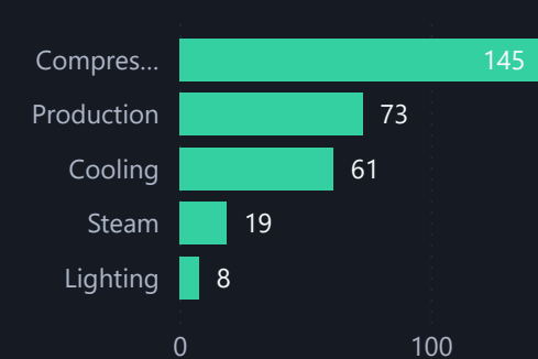
Equipment Category Load
