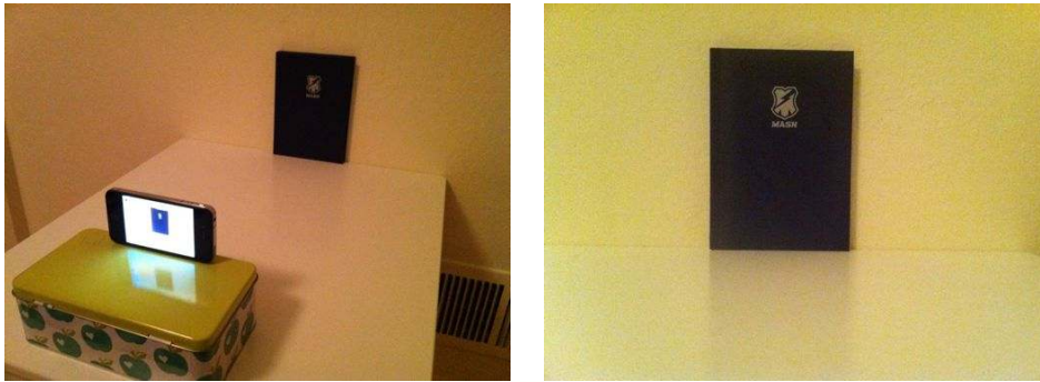
Figure 4.3: A simple camera calibration setup. (left) an image of the setup used. (right) the image used for the calibration. Measuring the width and height of the calibration object in the image and the physical dimensions of the setup is enough to determine the focal length.
