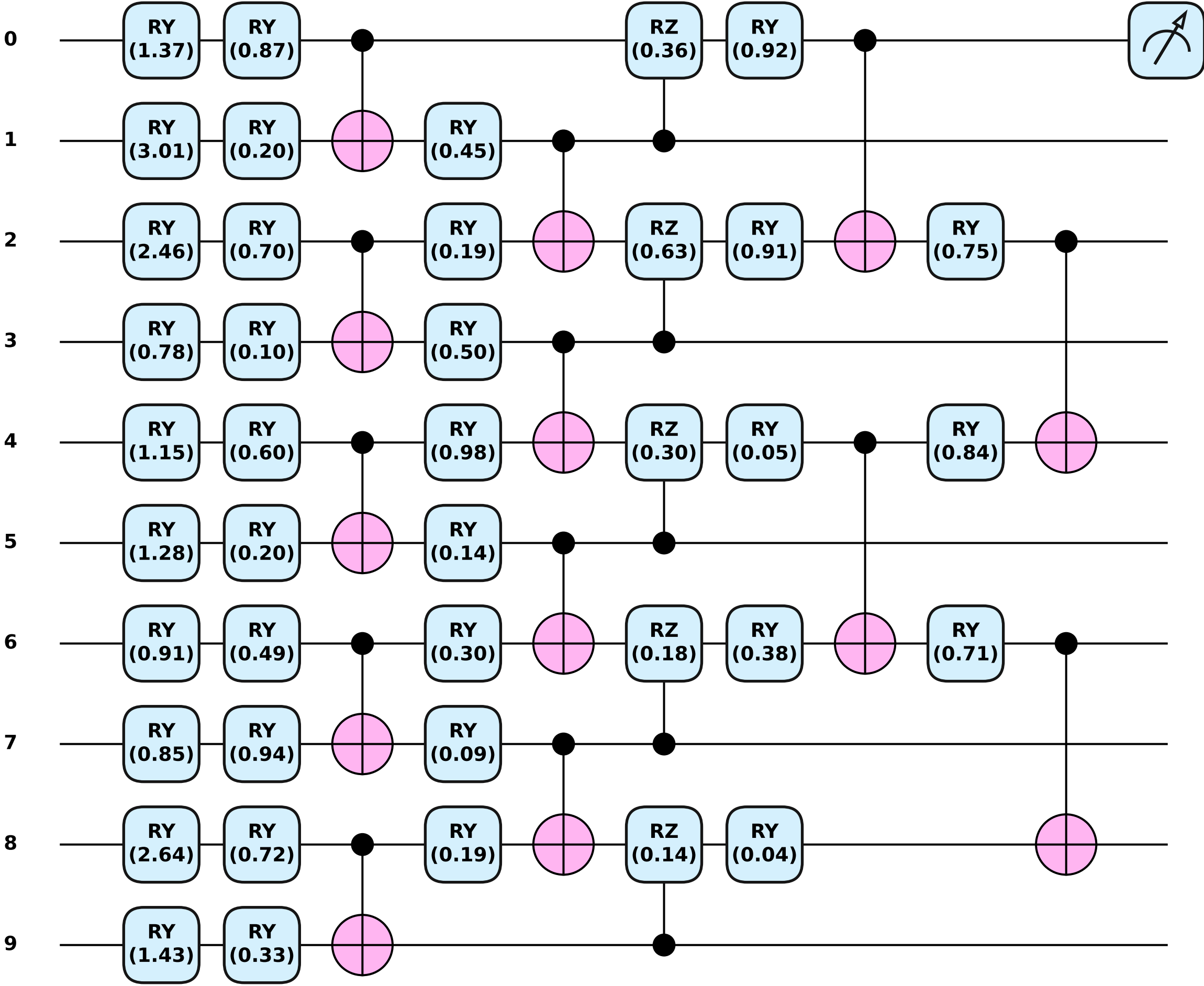
QCNN-Hybrid quantum head (10 qubits)
