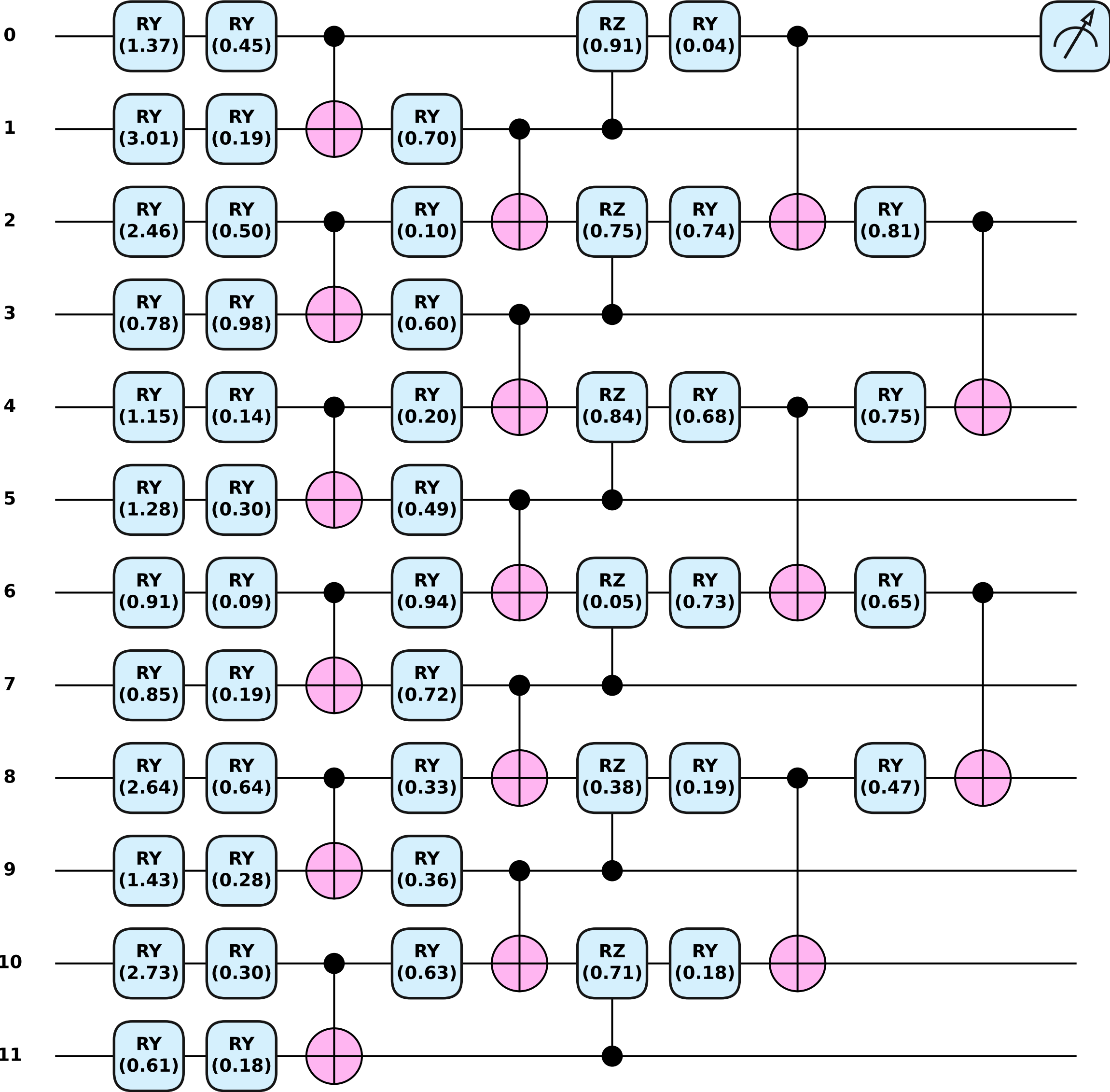
QCNN-Cong quantum circuit (12 qubits)
