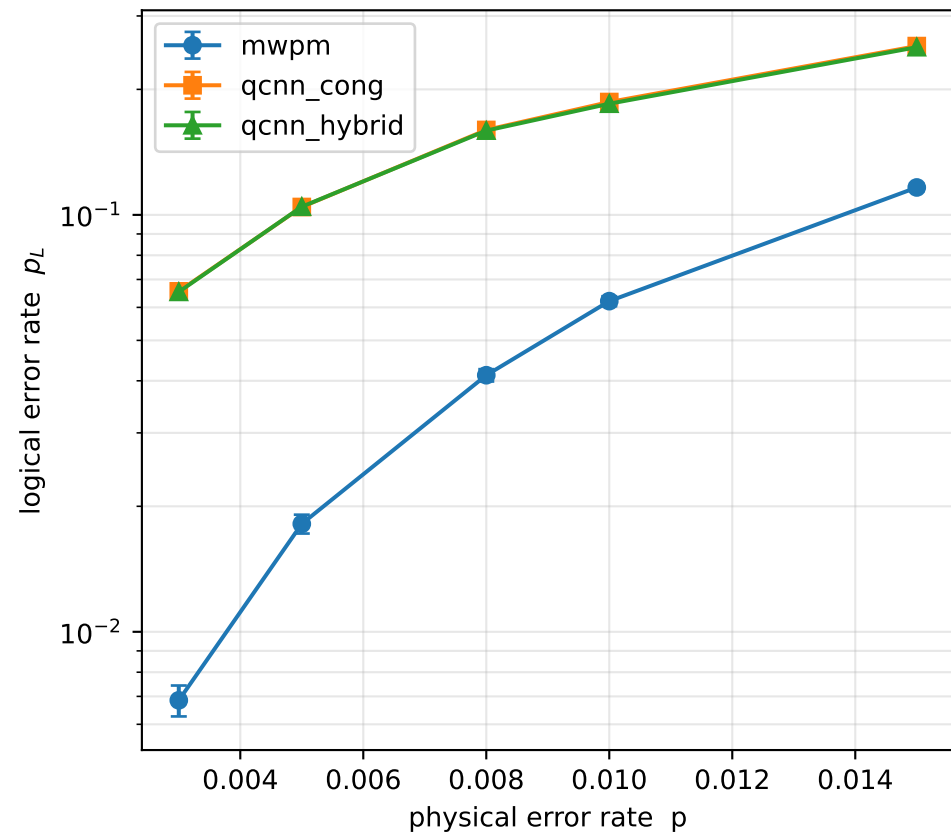
Decoder comparison (shots=20000) mwpm \Lambda=1.34 qcnngong \Lambda=0.68 qcnngybrid \Lambda=0.68
