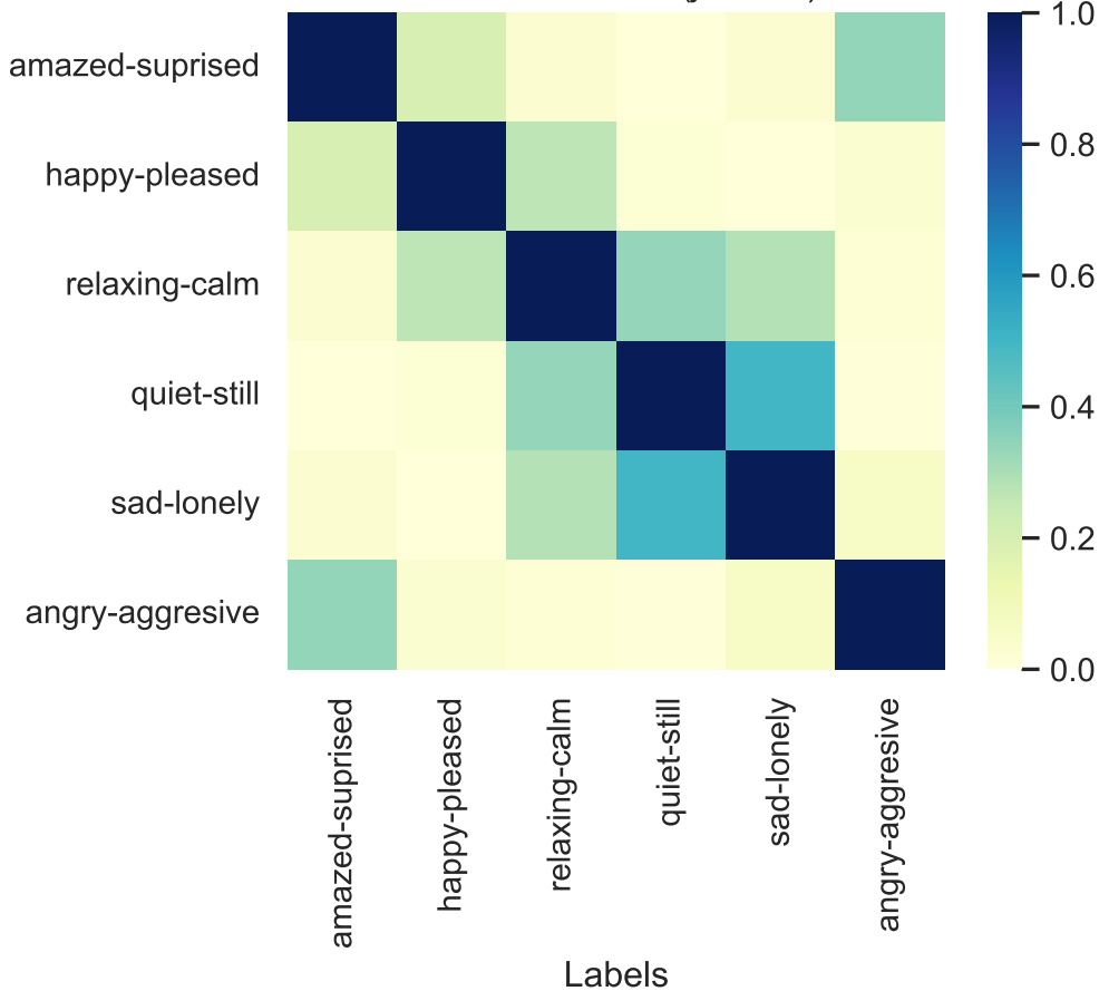
Pairwise Association Matrix (jaccard) - emotions
