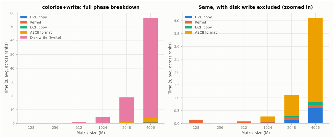
Figure 7: colorize+write split into its 5 phases vs. grid size. Left: full stack (write’s dominance is the point, not log-scaled). Right: same data with write excluded, zoomed in.
