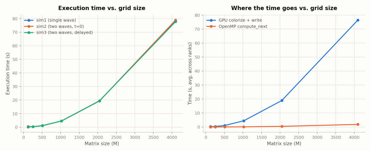
Figure 6: Execution time and its GPU/OpenMP split, varying grid size M (4 threads, 3 ranks sharing 1 GPU).
