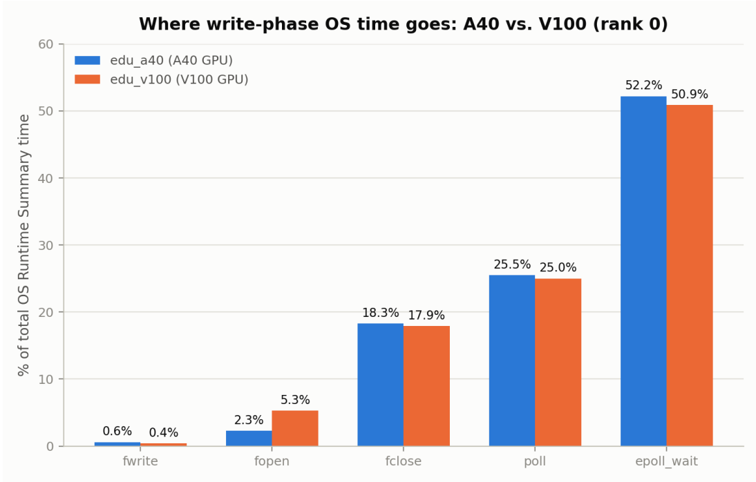
Figure 8: OS Runtime Summary breakdown (rank 0), edu_a40 vs. edu_v100 – nearly identical despite very different GPU hardware.
