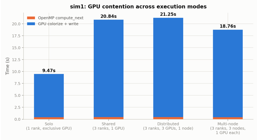
Figure 11: sim1’s execution time across four GPU/node sharing configurations, identical workload.
