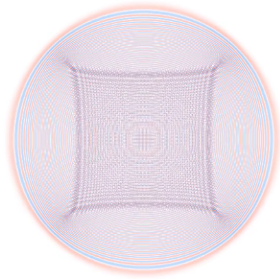
Figure 5: A rendered frame (sim1, late in the simulation): bright extrema, fading fronts, white calm regions.
