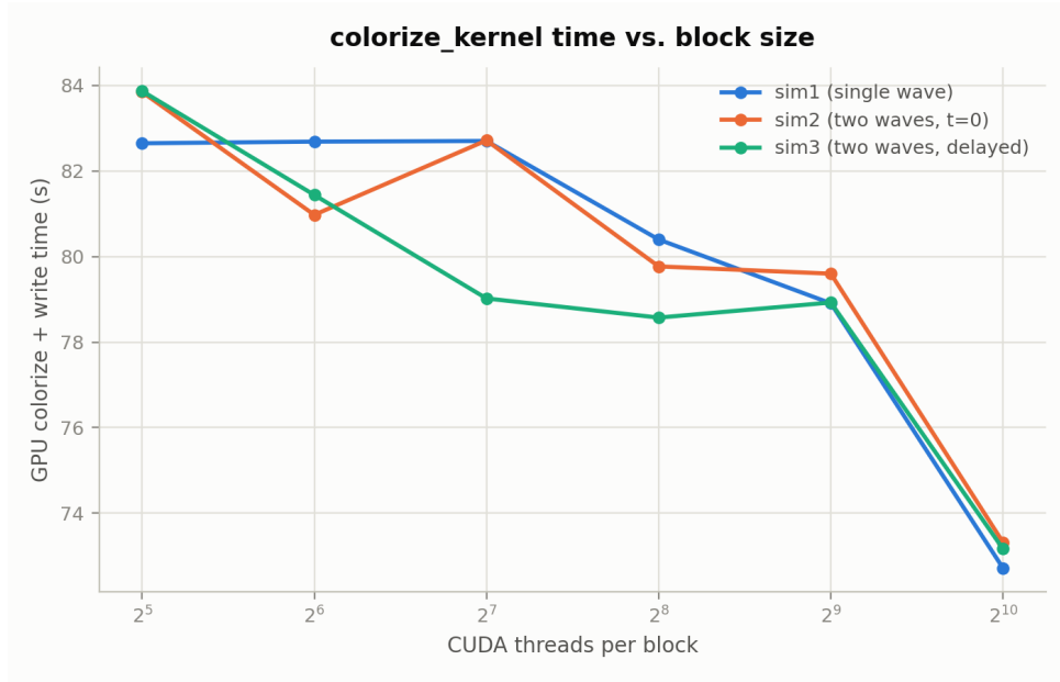
Figure 10: GPU colorize+write time vs. CUDA threads-per-block, M = 4096 .
