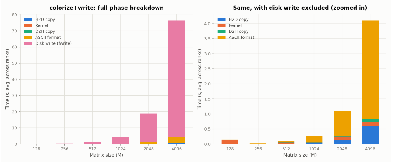
Figure 8: colorize+write split into its 5 phases vs. grid size. Left: full stack (write’s dominance is the point, not log-scaled). Right: same data with write excluded, zoomed in.
