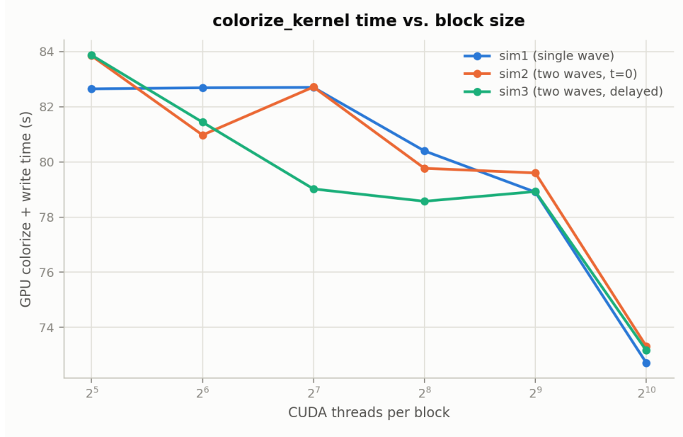
Figure 11: GPU colorize+write time vs. CUDA threads-per-block, M = 4096 .
