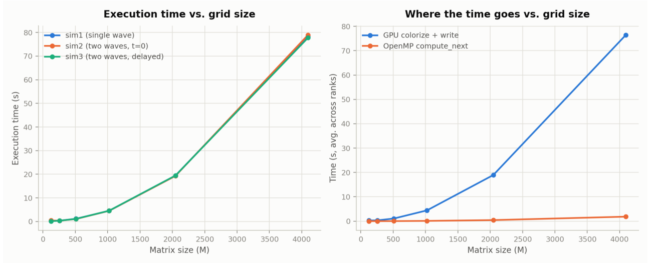
Figure 7: Execution time and its GPU/OpenMP split, varying grid size M (4 threads, 3 ranks sharing 1 GPU).
