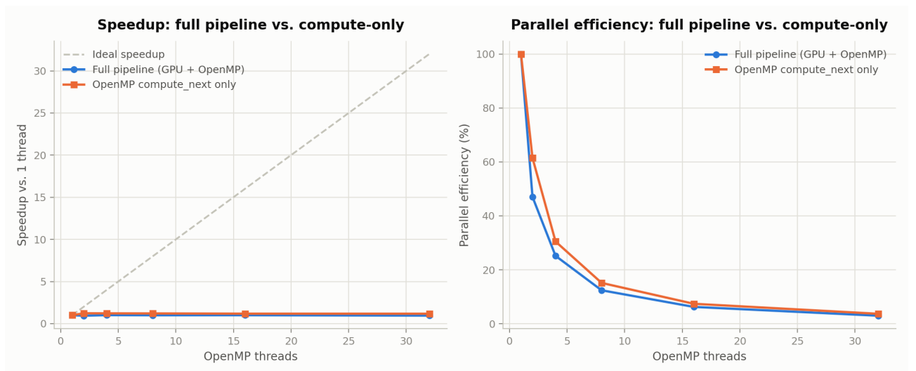
Figure 10: Speedup and efficiency vs. OpenMP thread count at M = 4096 , full pipeline vs. compute-only.
