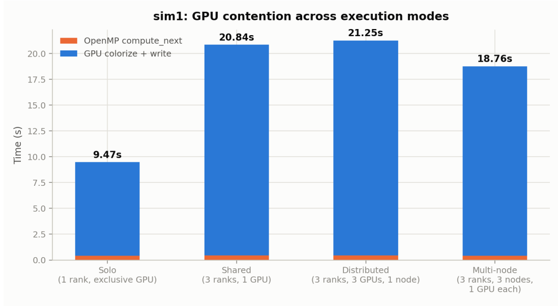
Figure 12: sim1’s execution time across four GPU/node sharing configurations, identical workload.
