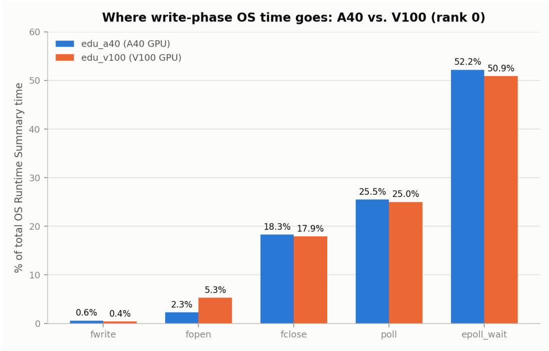
Figure 9: OS Runtime Summary breakdown (rank 0), edu_a40 vs. edu_v100 – nearly identical despite very different GPU hardware.
