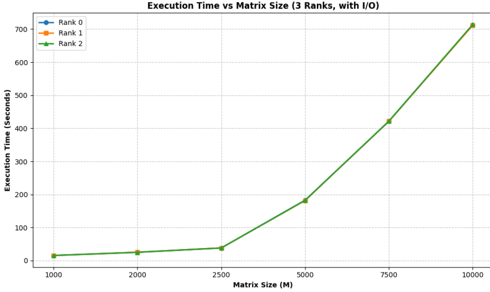
Figure 5: Execution Time vs Matrix Size.
