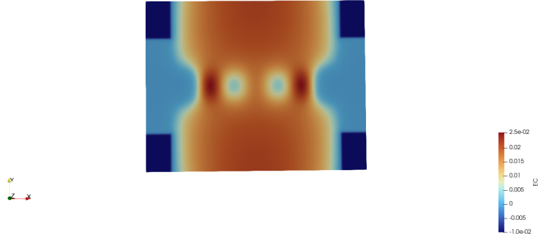
Figure 4.1: Density charge map (Slice at z=45 ) showing the double quantum dot region.
