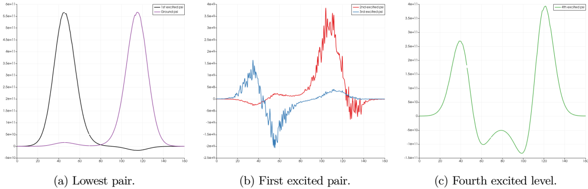
Figure 3.7: Signed wavefunction profiles along the axis connecting the two dots.
