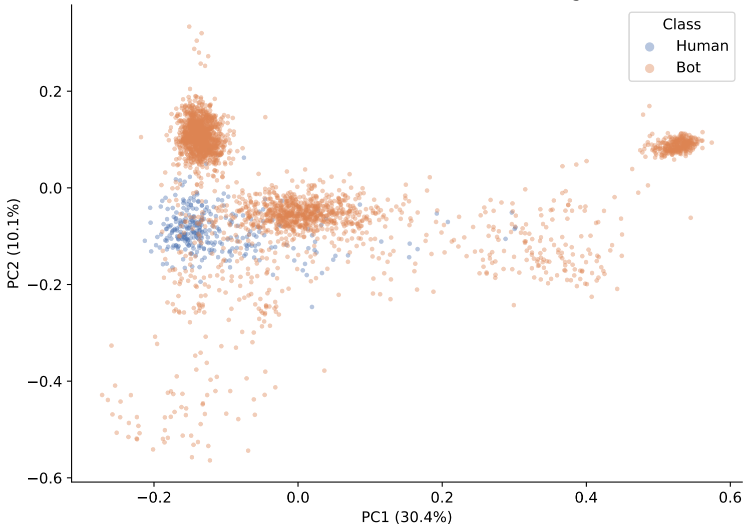
PCA of Mean Tweet Sentence Embeddings
