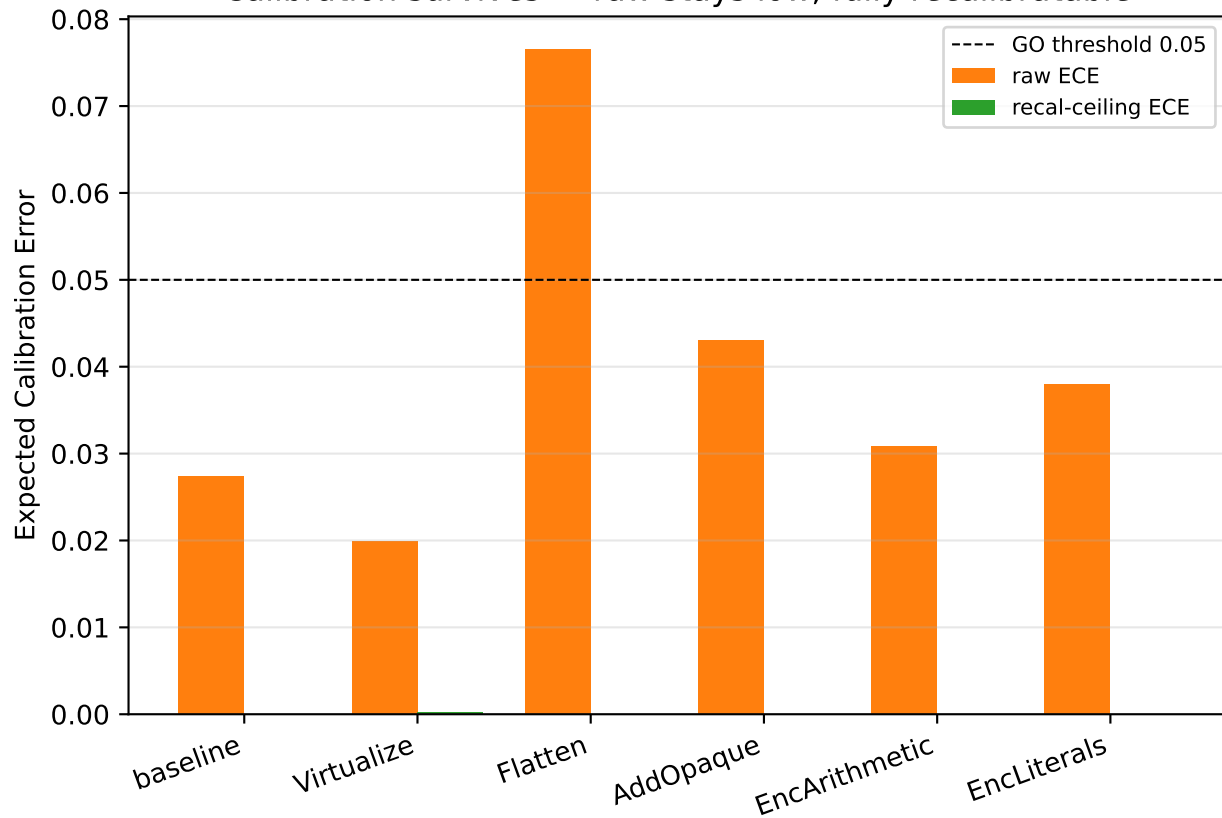
Calibration survives — raw stays low, fully recalibratable
