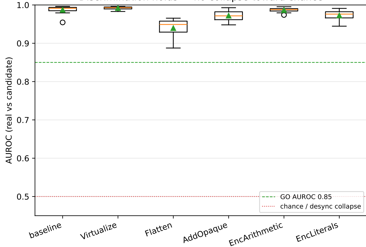
Discrimination holds — no collapse toward chance
