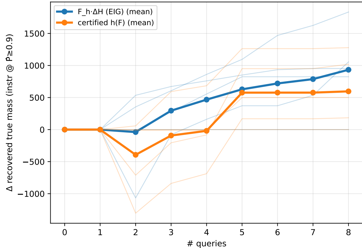
Effort curve — decoy arm
