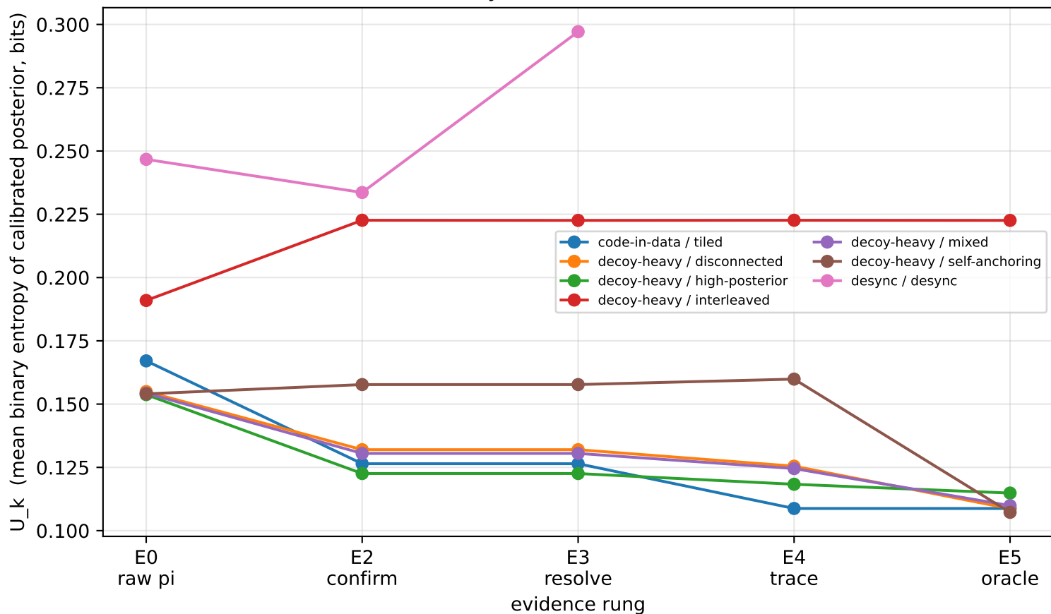
Recoverability staircase (instruction-start)
