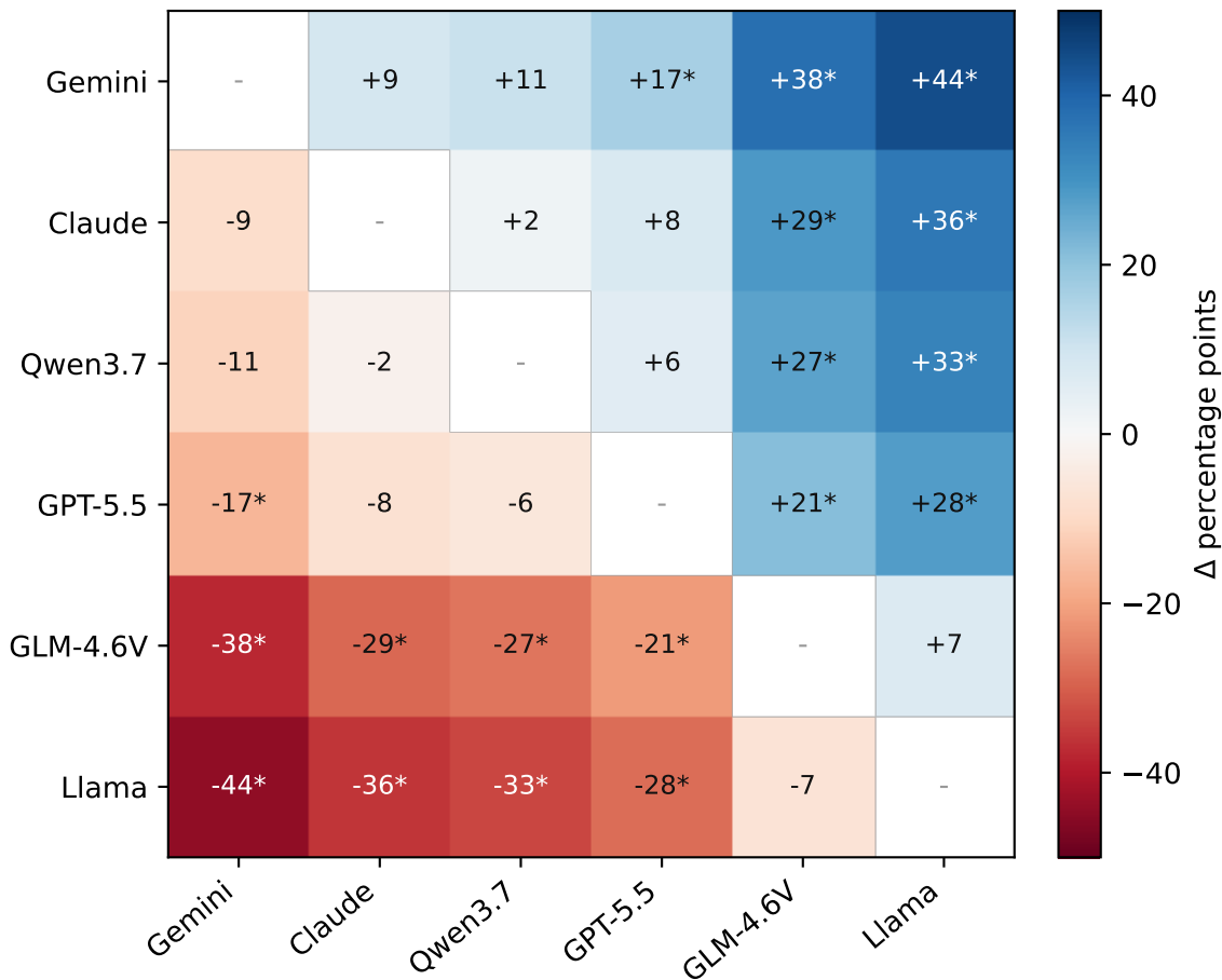
Pairwise pass-rate difference (row – column), * = Holm p < 0.05
