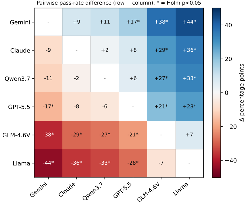
Figure 4: Pairwise pass-rate differences (row minus column, percentage points); an asterisk marks a Holm-corrected McNemar p < 0.05 .
