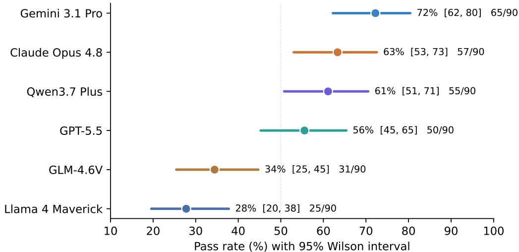
Figure 2: Pass rate by model with 95% Wilson intervals over the 90 images. The top three intervals overlap; the ordering within that cluster is not statistically resolved.
