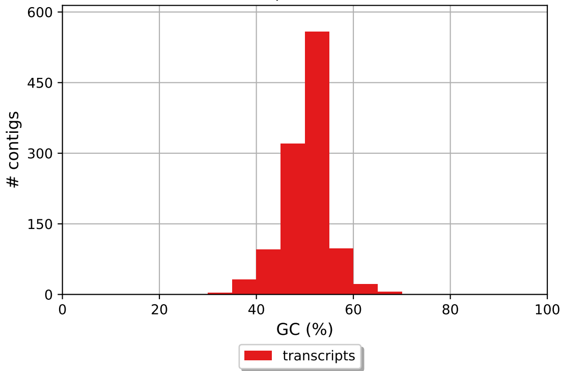
transcripts GC content
