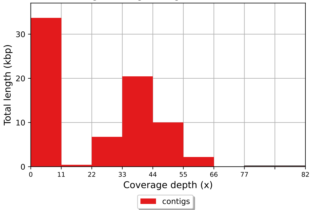
contigs coverage histogram (bin size: 11x)
