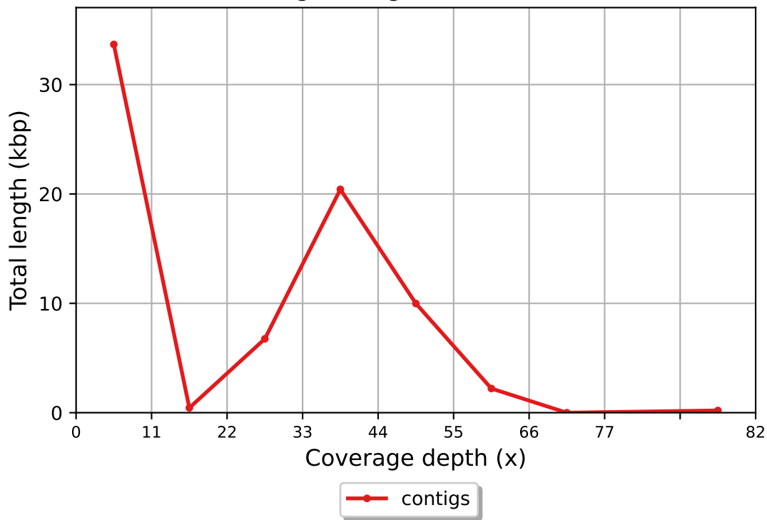
Coverage histogram (bin size: 11x)
