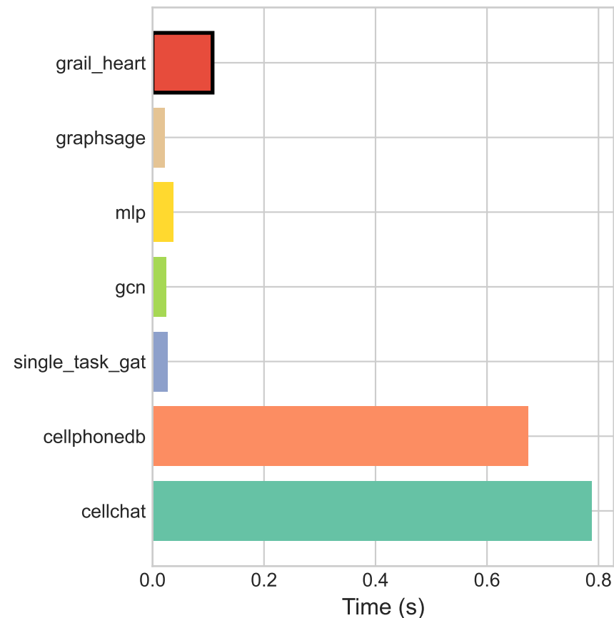
Inference Time
