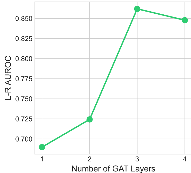
L-R Prediction Performance
