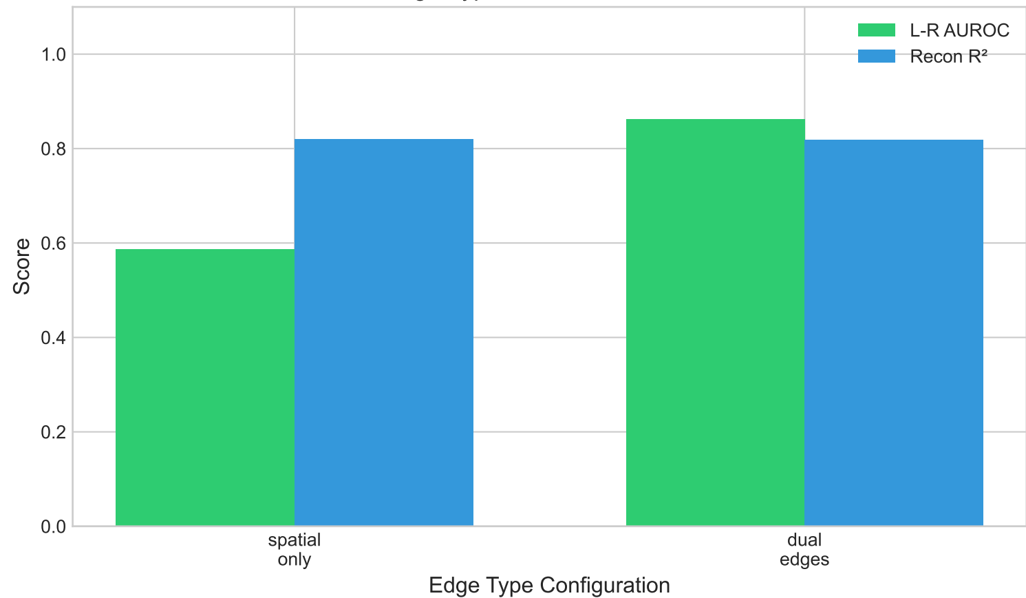
Edge-Type Awareness Ablation
