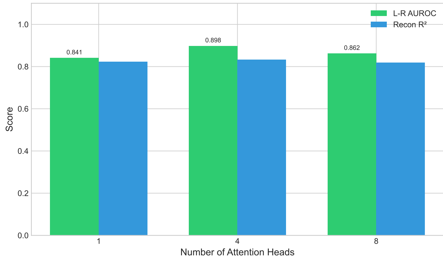
Effect of Attention Heads on Performance
