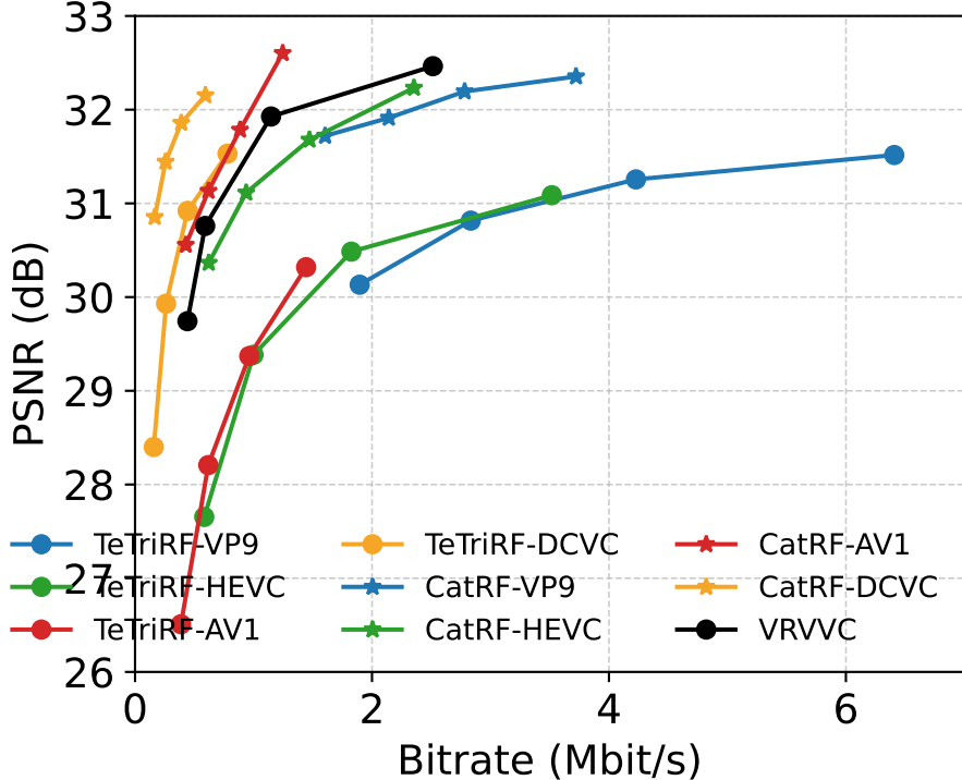
TriPlane video RD curves
