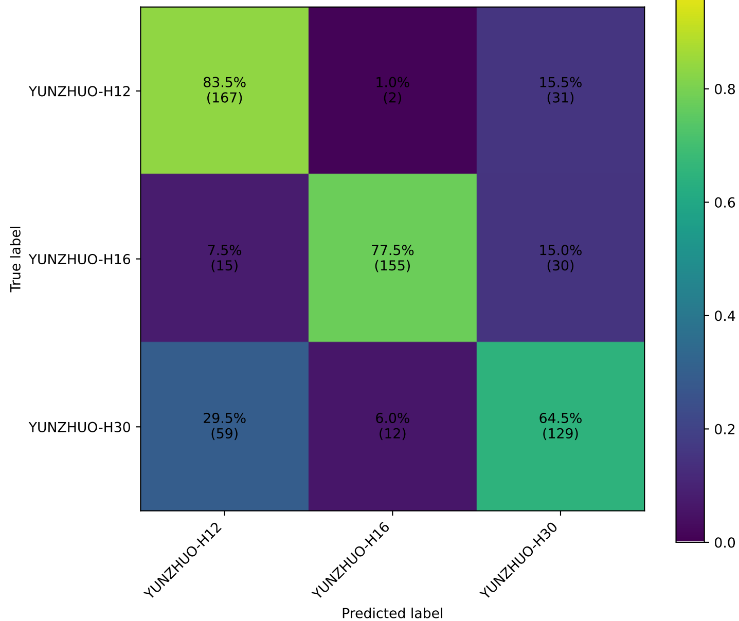
Normalized FFT-based UAV Classifier Confusion Matrix
