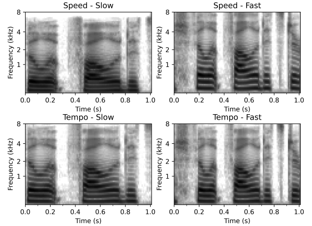
Figure 1: The log-Mel spectrogram representations of the same 1-second speech segment at the very slow and very fast settings of speed and tempo.
