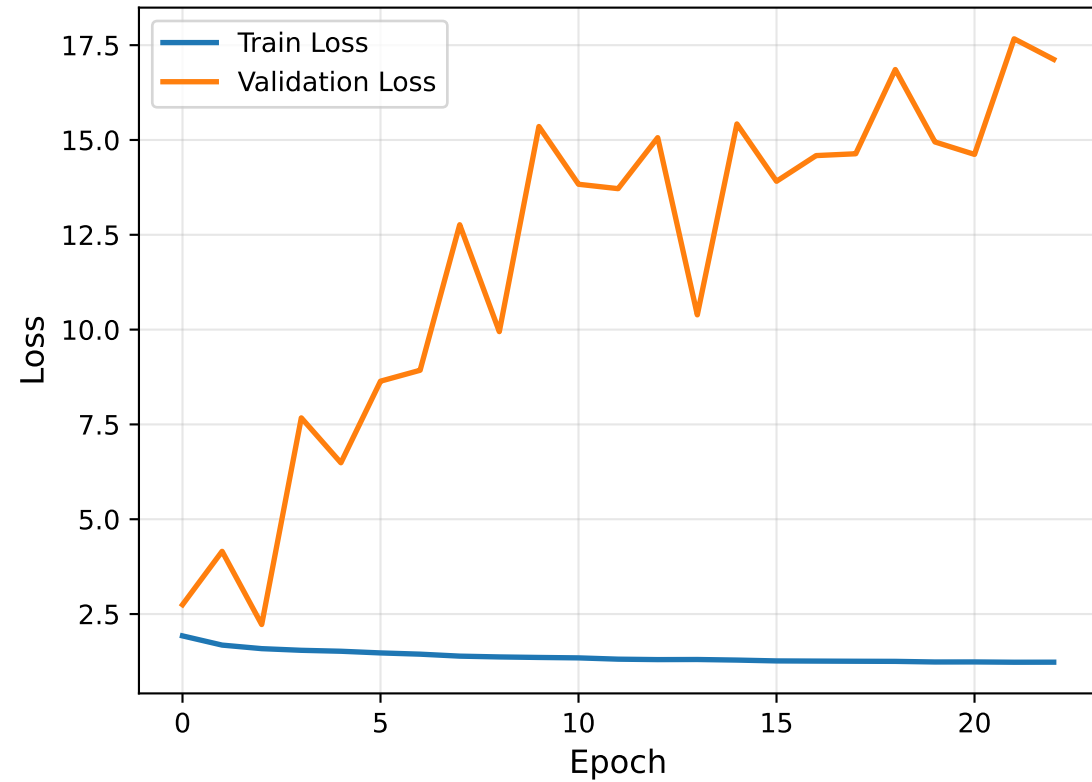
resnet18 - Training History
