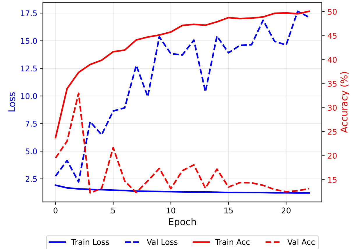
resnet18 - Combined View
