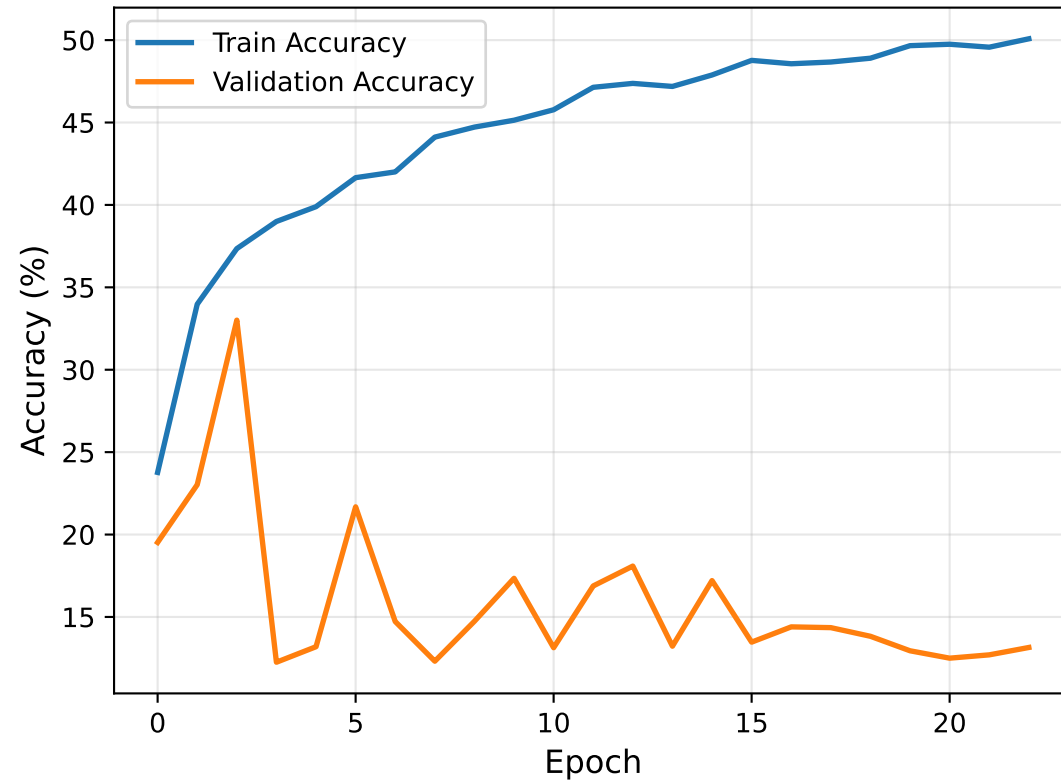
resnet18 - Accuracy Progress
