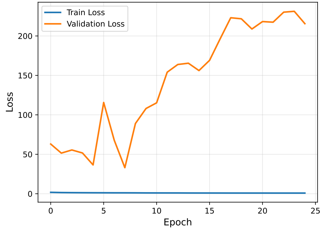
resnet18 - Training History
