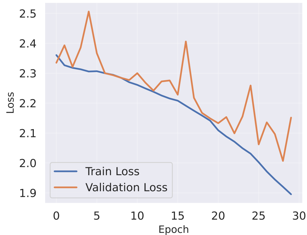
resnet18 - Training History
