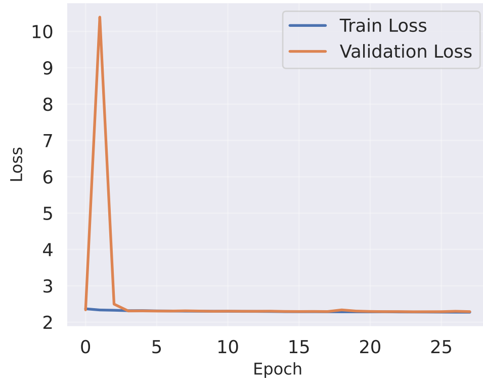
resnet18 - Training History
