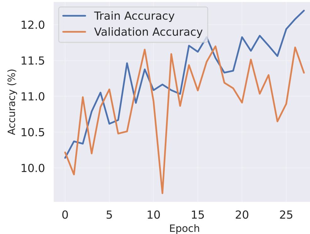
resnet18 - Accuracy Progress
