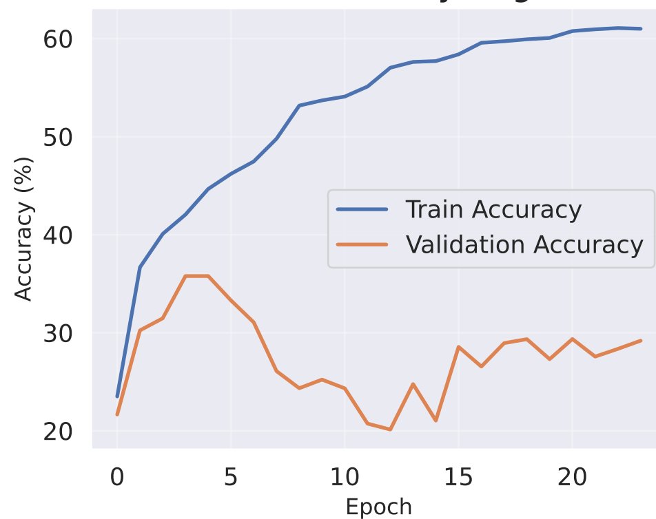
resnet18 - Accuracy Progress
