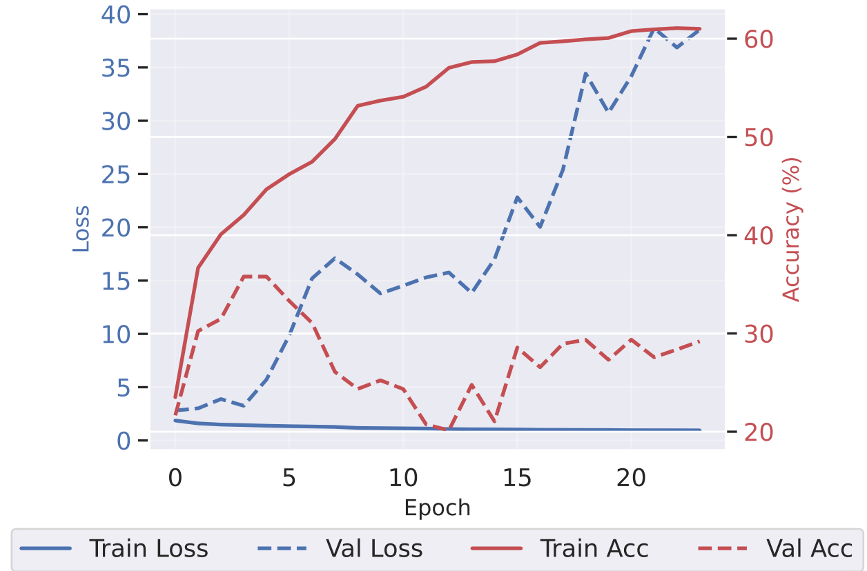
resnet18 - Combined View
