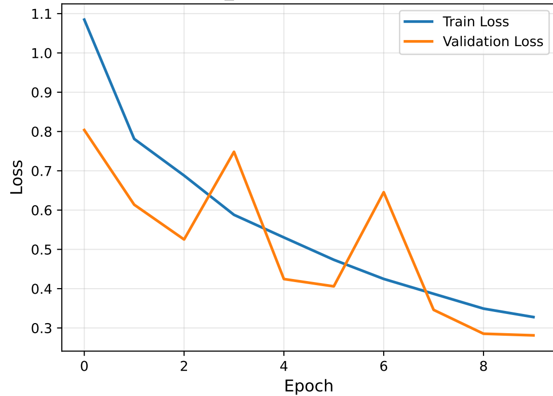
simple_cnn - Training History
