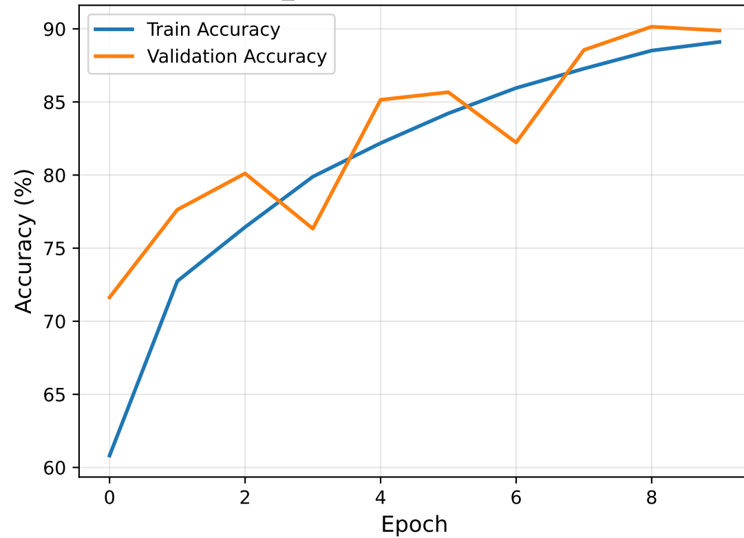
simple_cnn - Accuracy Progress
