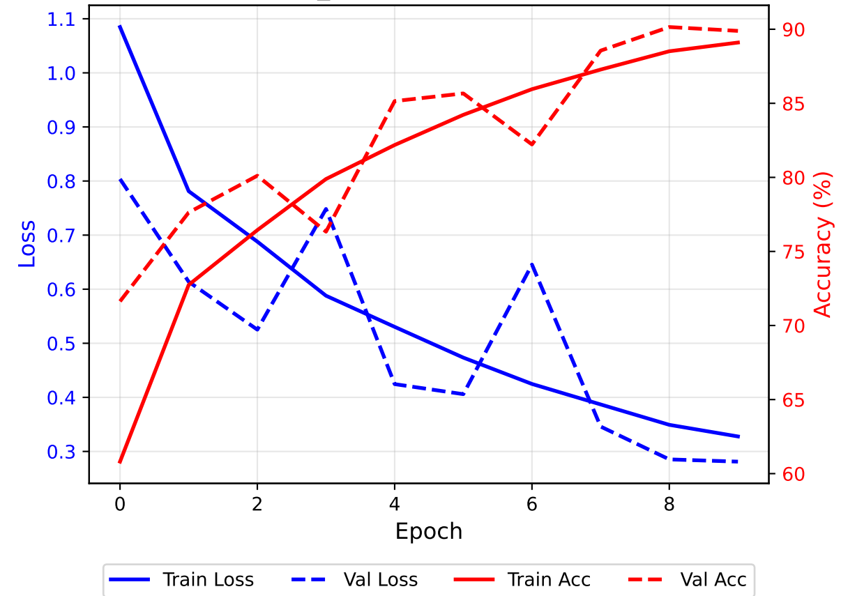
simple_cnn - Combined View
