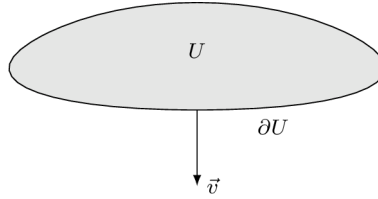
Figure 1.2: Outward derivative.
