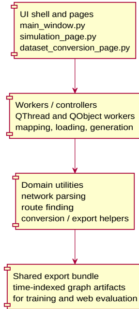
Figure 3: Desktop software structure (component view). UI pages delegate heavy work to asynchronous workers, which call utility/service modules and produce a shared export bundle.
