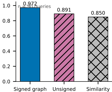
Coalition purity
