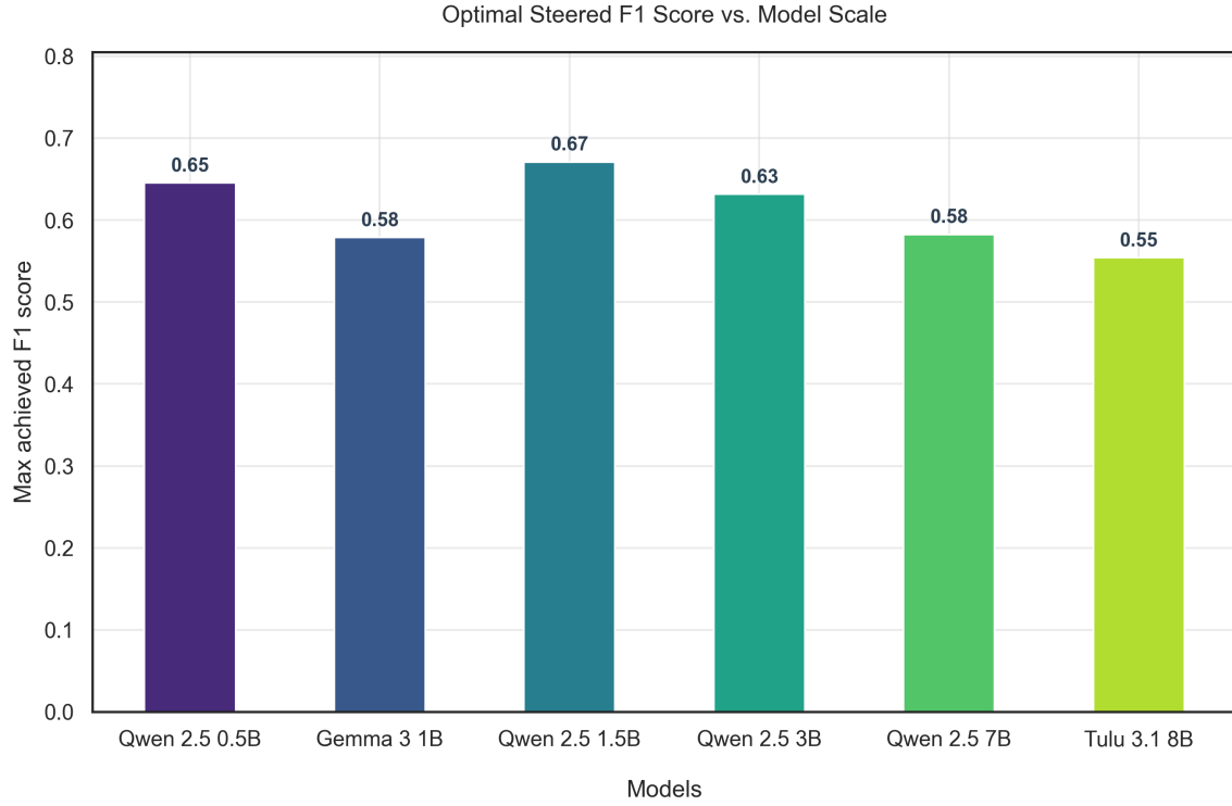
Figure 1: Peak mean F1 for each model at its best tested layer-coefficient pair.
