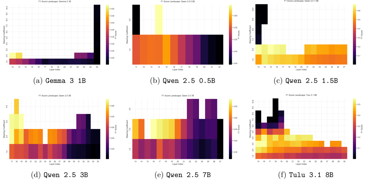
Figure 5: Representative F1 heatmaps over layer and coefficient. Brighter regions indicate higher mean F1. Note that Gemma 3 1B shows earlier collapse at higher coefficients compared to Qwen models. [cite: 24, 25]
