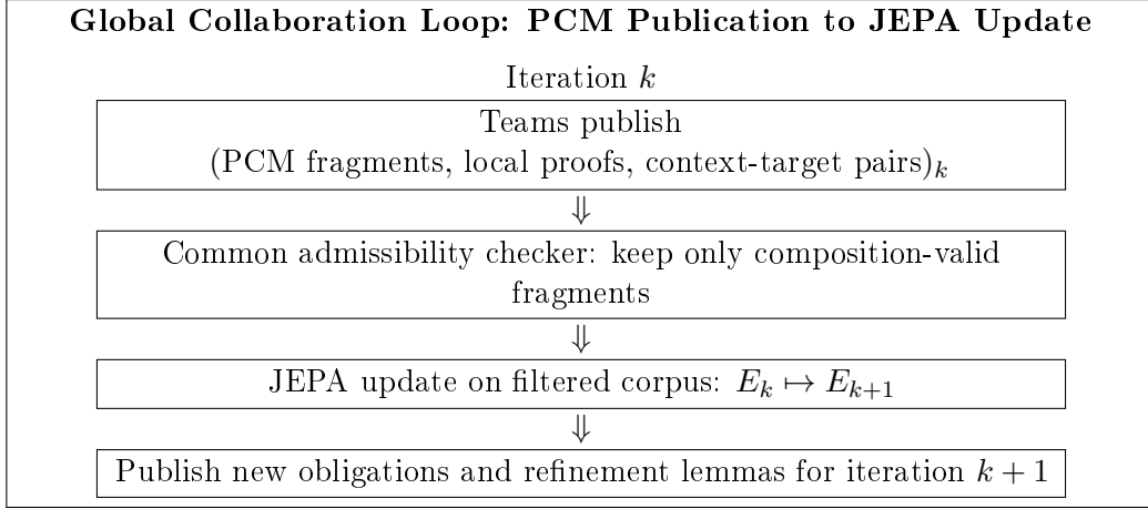
Figure 2: Indicative training-governance cycle. The loop emphasizes co-evolution: representation quality improves statistically while composition guarantees improve constructively.
