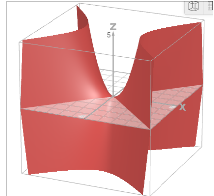
Figure 3.3.1: Saddle point
