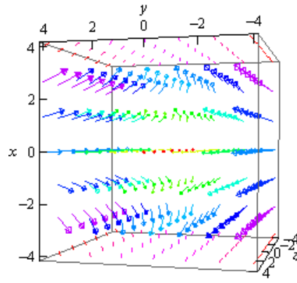
(b) \vec{F}(x, y, z) = 2x\hat{i} - 2y\hat{j} - 2x\hat{k}
